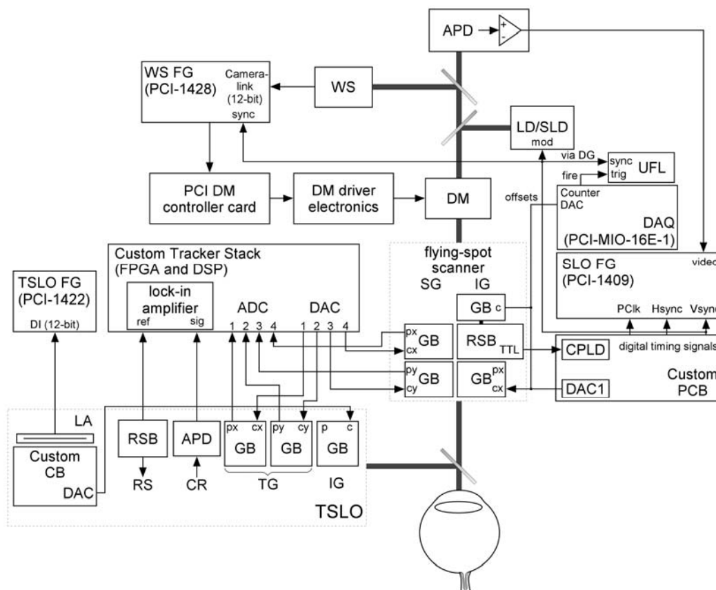
Figure 4: Instrumentation and electronics for the TAOSLO system.
