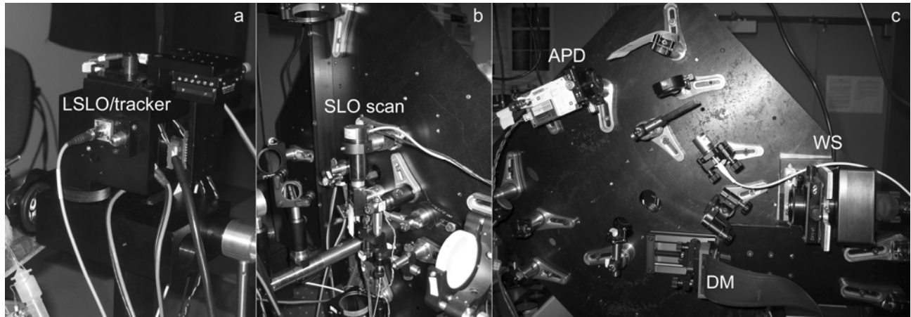
Figure 2: Photographs of (a) retinal tracking head, (b) AOSLO front plate, and (c) AOSLO back plate.
